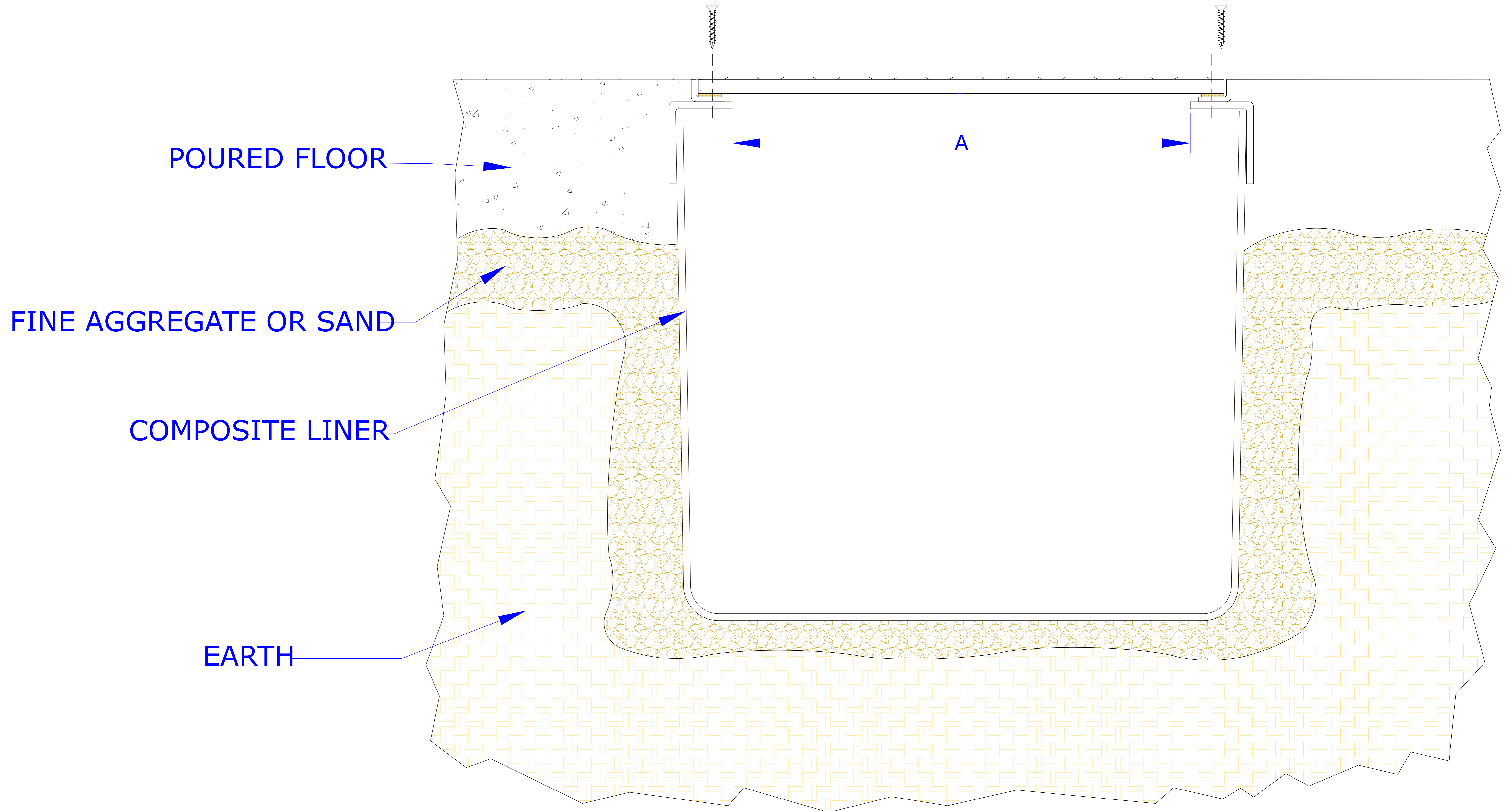
Model CLL Installation Detail
