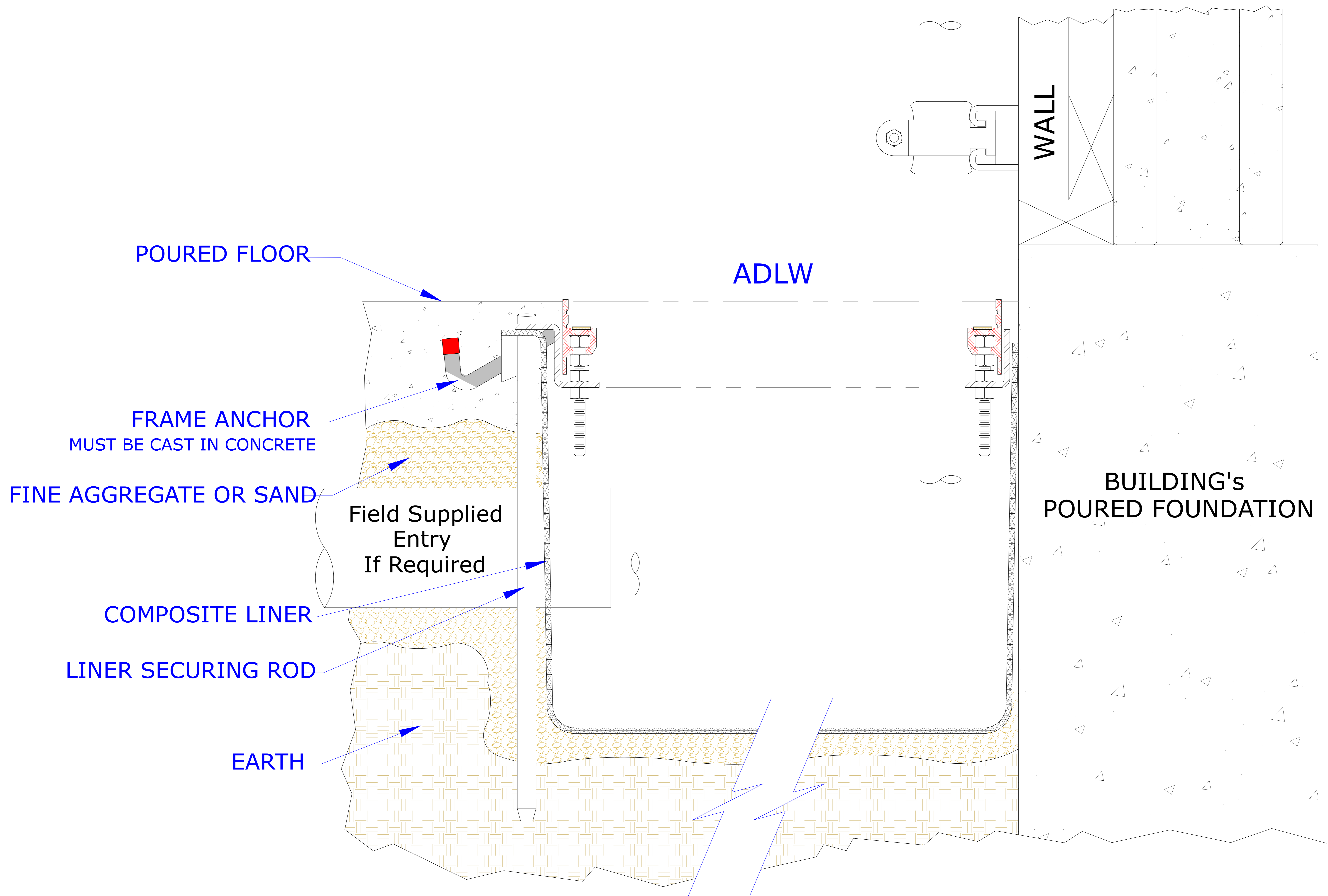
Model ADL-W Installation Detail
